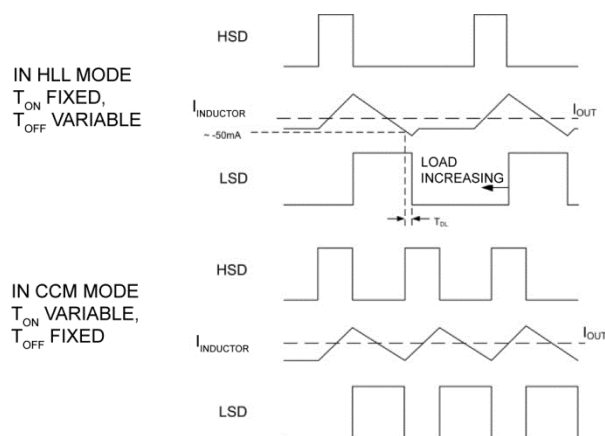
Figure 2. Signals for High-Side Switch Drive (HSD) for T_{\text{ON}} Control, Inductor Current, and Low-Side Switch Drive (LSD) for T_{\text{OFF}} Control
