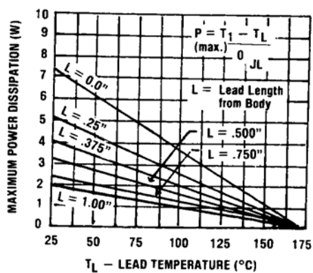
FIGURE 3 MAXIMUM POWER DISSIPATION vs LEAD TEMPERATURE
