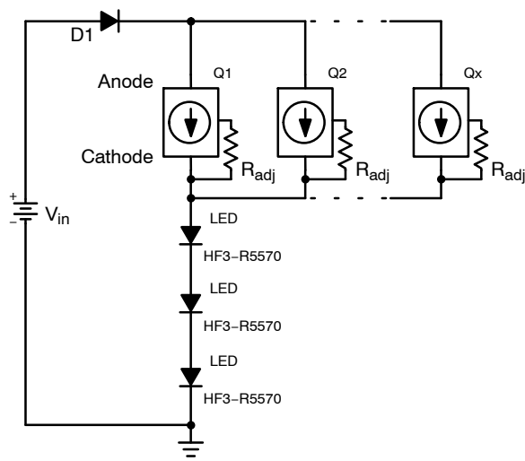
Figure 9. Typical Application Circuit (90 mA each LED String)
