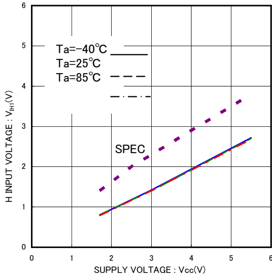
Fig.5 'H' input voltage V_{IH1} (SCL1, SCL2, SDA1, SDA2, WP2)
