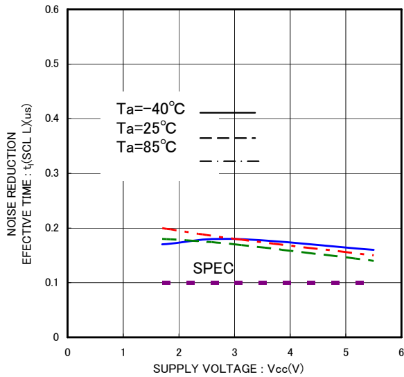
Fig.29 Noise reduction effective time t_i(\text{SCL L})
