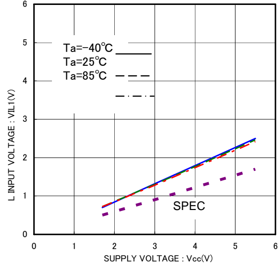
Fig.6 'L' input voltage V_{IL1} (SCL1, SCL2, SDA1, SDA2, WP2)
