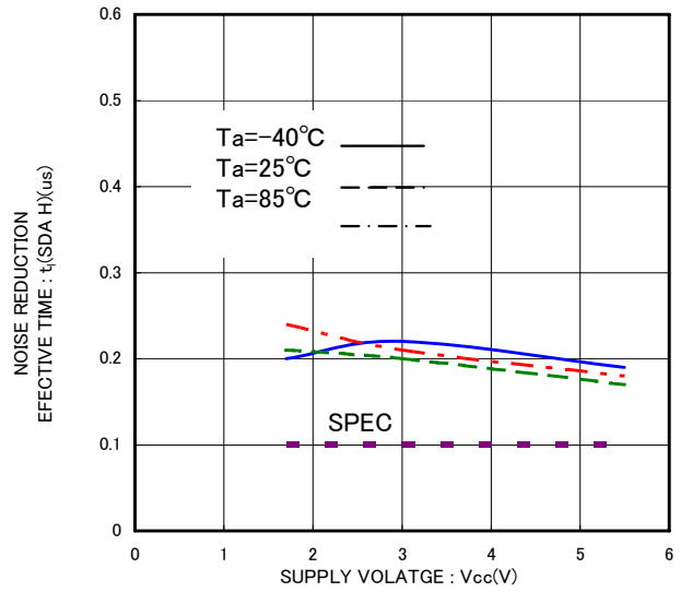
Fig.30 Noise resuction effective time t_i(\text{SDA H})
