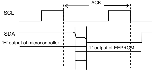
Over current flows to SDA line by 'H' output of microcontroller and 'L' output of EEPROM. Fig.53-(b) Input / output collision timing
