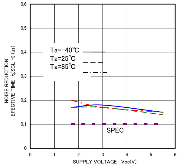
Fig.28 Noise reduction effective time t_t(\text{SCL H})
