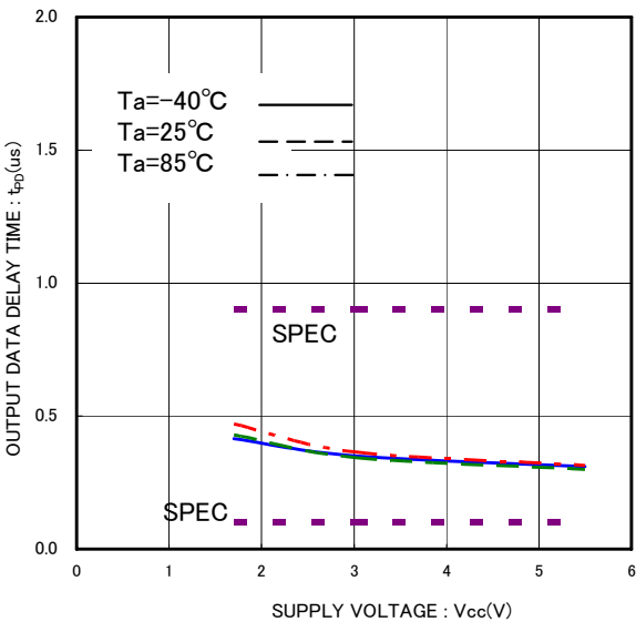
Fig.24 'H' Data output delay time t_{PD1}
