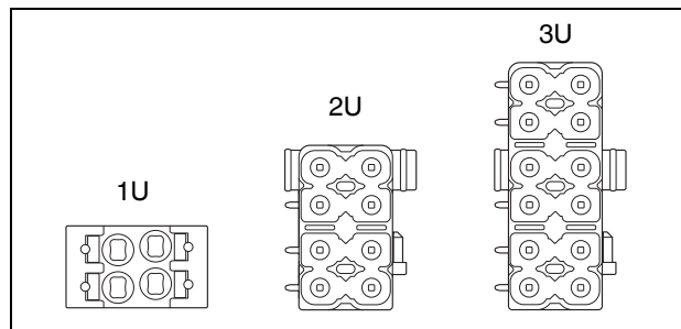
Figure 3 1U connector and 2U + 3U headers
