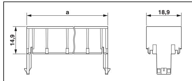
Figure 9 Dimensions of the housing cover
