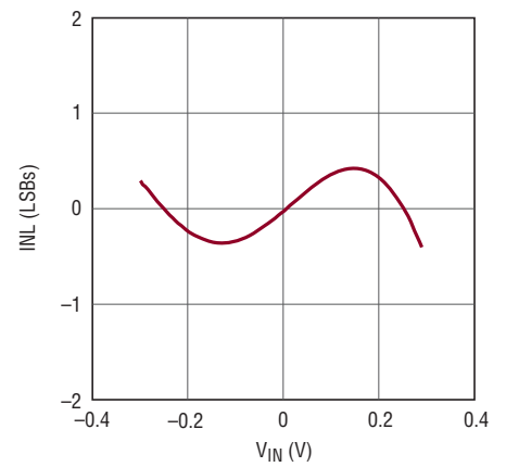
Differential INL
