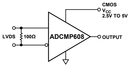
Figure 13. LVDS-to-CMOS Receiver
