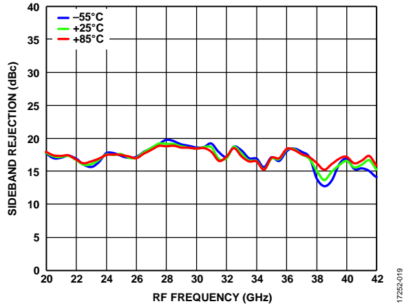
Figure 19. Sideband Rejection vs. RF Frequency at Various Temperatures, LO Drive = 18 dBm
