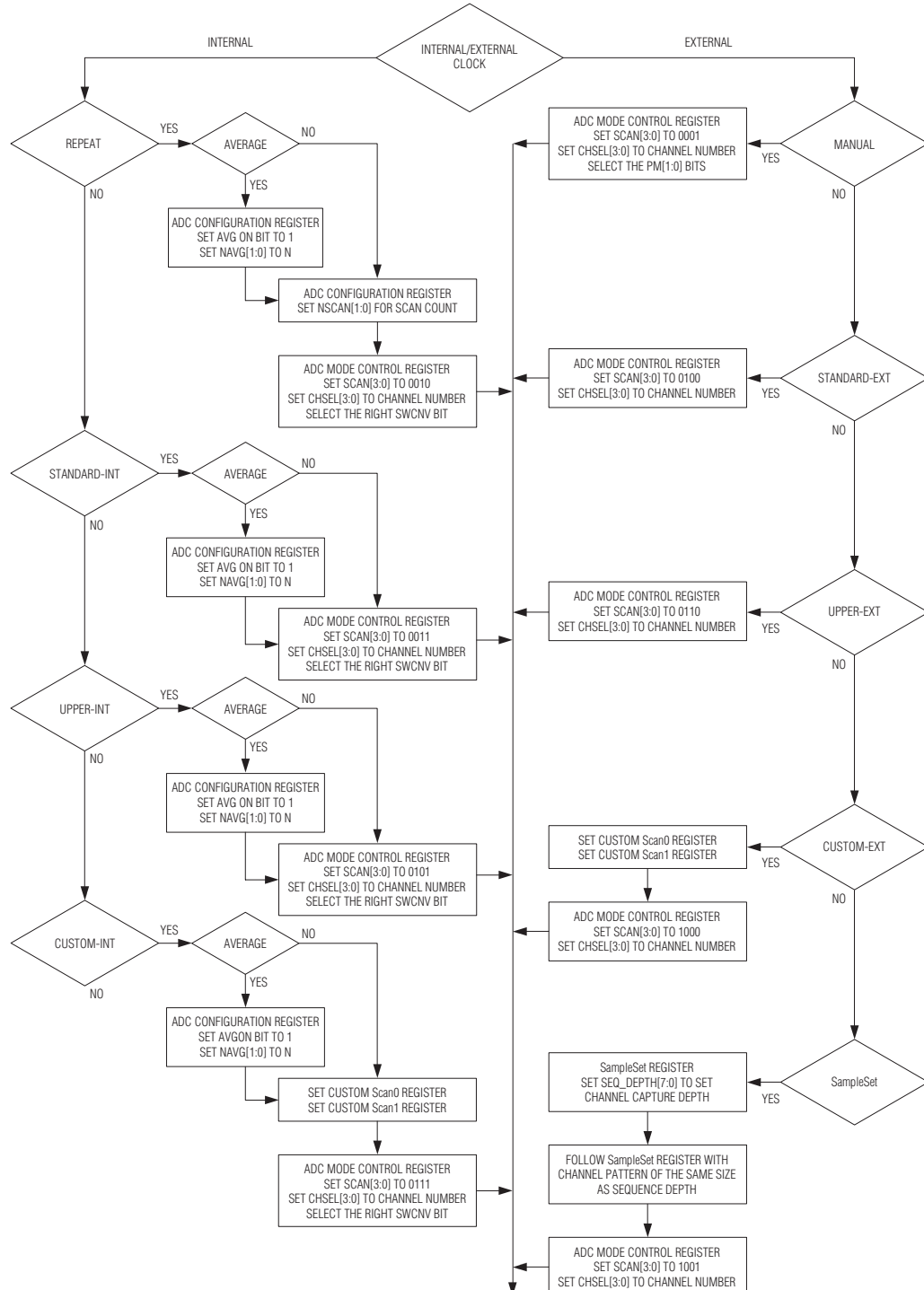
Figure 12. ADC Mode Select Programming Sequence
