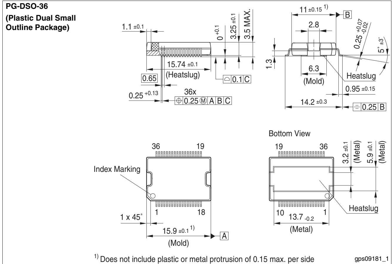
Figure 12 PG-DSO36
