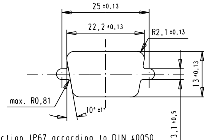
Panel Cutout
