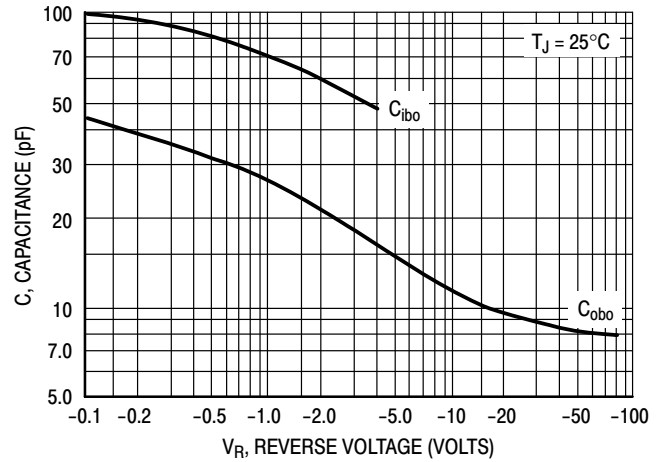
Figure 2. Capacitance
