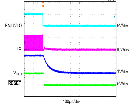
MAXM15467 SHUTDOWN THROUGH ENABLE V_{IN} = 12V , ADJUSTABLE V_{OUT} = 1.5V , FULL LOAD, PWM MODE
