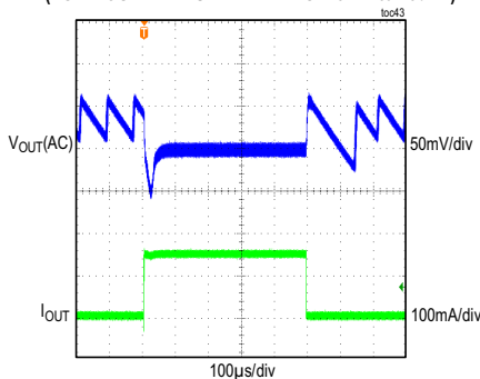
MAXM15467 LOAD TRANSIENT RESPONSE V_{IN} = 12V , ADJUSTABLE V_{OUT} = 1.5V , PFM MODE (LOAD CURRENT STEPPED FROM 5mA TO 150mA)
