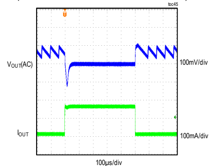
MAXM15467 LOAD TRANSIENT RESPONSE V_{IN} = 24V , ADJUSTABLE V_{OUT} = 3.3V , PFM MODE (LOAD CURRENT STEPPED FROM 5mA TO 150mA)
