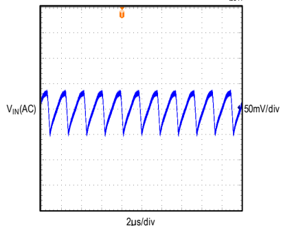
MAXM15465 INPUT VOLTAGE RIPPLE V_{IN} = 24V , FIXED V_{OUT} = 3.3V , FULL LOAD, PWM MODE
