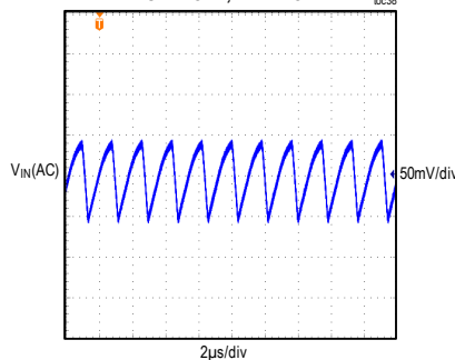
MAXM15467 INPUT VOLTAGE RIPPLE V_{IN} = 12V , ADJUSTABLE V_{OUT} = 1.5V FULL LOAD, PWM MODE
