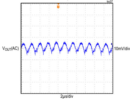
MAXM15466 OUTPUT VOLTAGE RIPPLE V_{IN} = 24V , FIXED V_{OUT} = 5V FULL LOAD, PWM MODE
