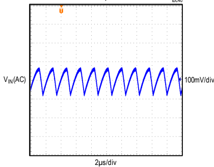
MAXM15467 INPUT VOLTAGE RIPPLE V_{IN} = 24V , ADJUSTABLE V_{OUT} = 5V , FULL LOAD, PWM MODE
