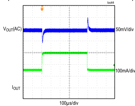
MAXM15467 LOAD TRANSIENT RESPONSE V_{IN} = 12V , ADJUSTABLE V_{OUT} = 1.5V , PWM MODE (LOAD CURRENT STEPPED FROM 150mA TO 300mA)
