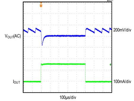
MAXM15466 LOAD TRANSIENT RESPONSE V_{IN} = 24V , FIXED V_{OUT} = 5V , PFM MODE (LOAD CURRENT STEPPED FROM 5mA TO 150mA)
