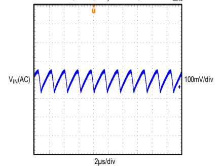
MAXM15466 INPUT VOLTAGE RIPPLE V_{IN} = 24V , FIXED V_{OUT} = 5V FULL LOAD, PWM MODE
