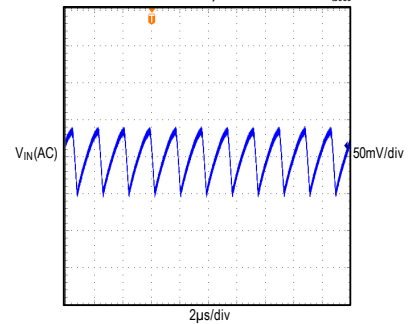
MAXM15467 INPUT VOLTAGE RIPPLE V_{IN} = 24V , ADJUSTABLE V_{OUT} = 3.3V , FULL LOAD, PWM MODE
