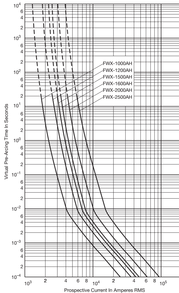
Time-Current Curve
