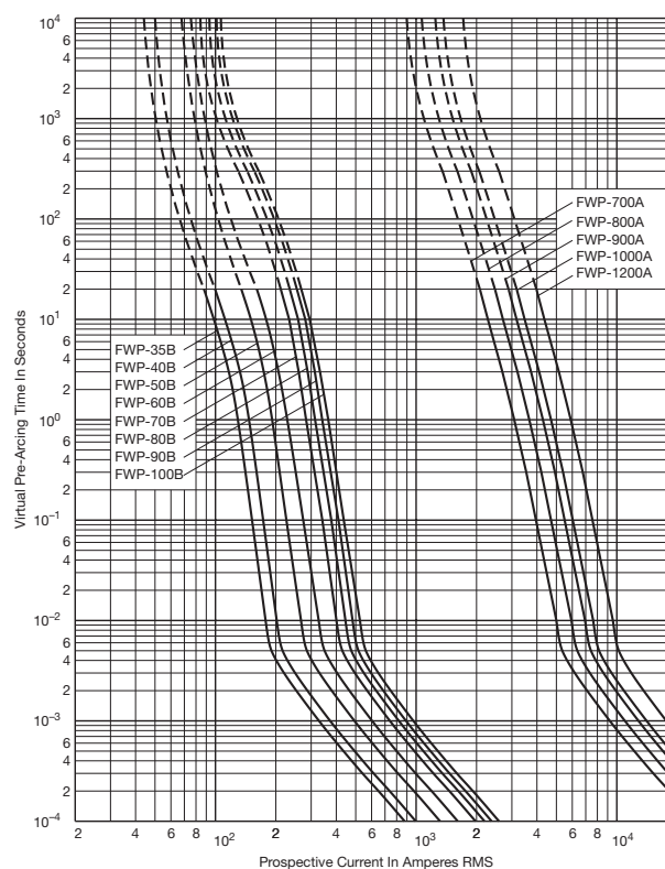
Time-Current Curve
