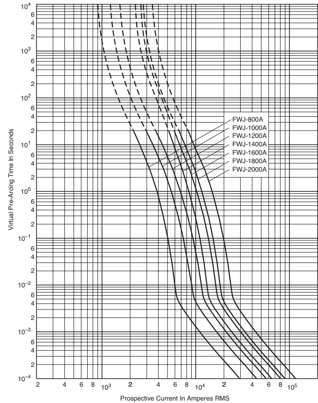
Time-Current Curve
