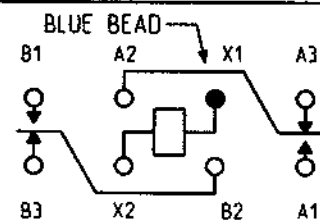
TERMINAL VIEW
