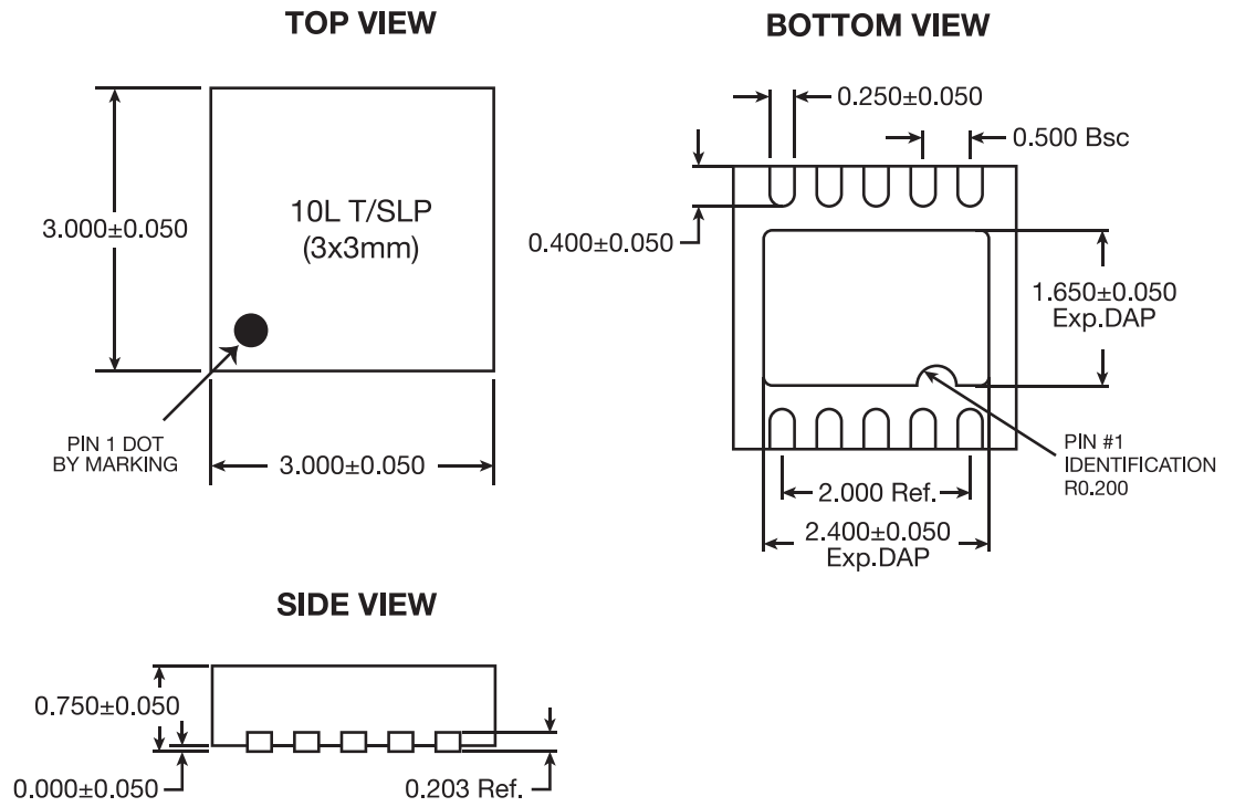
Figure 8: Package drawing of 10-lead, 3mm x 3mm DFN
