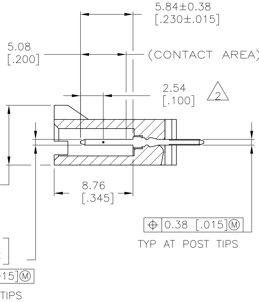
SECTION X-X
