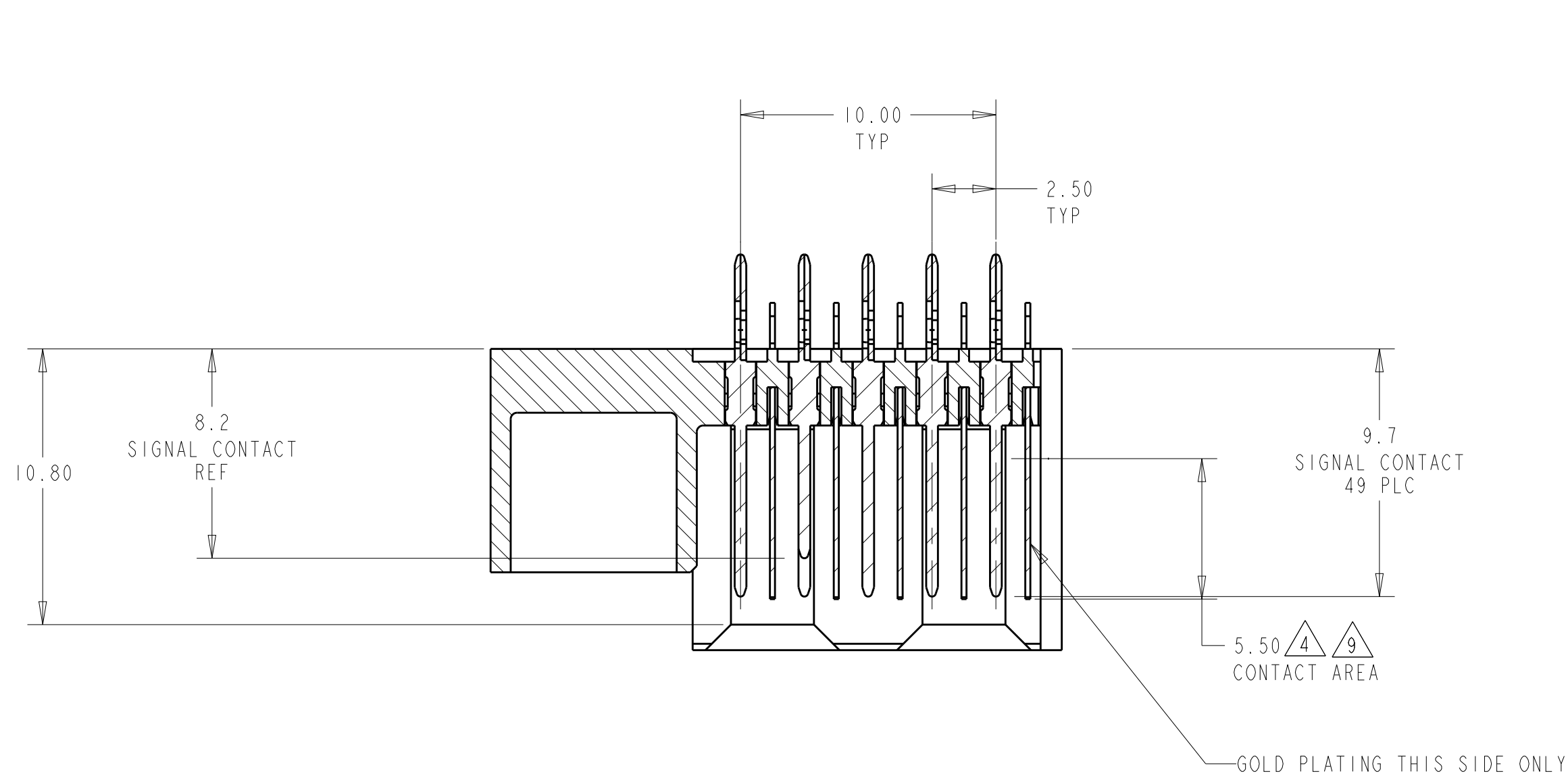
SECTION B-B
