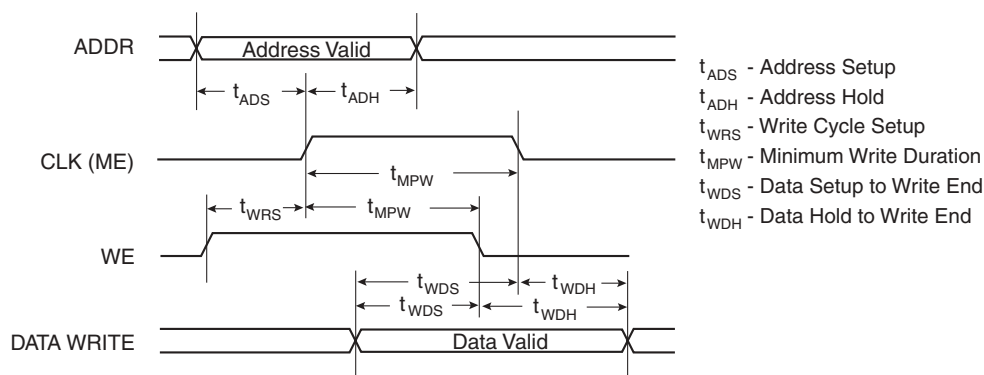
Figure 84. SRAM Write Cycle Timing Diagram
