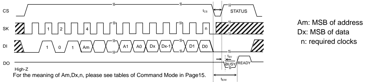
Figure 36. Write Cycle
