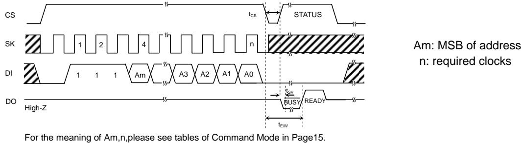
Figure 39. Erase Cycle
