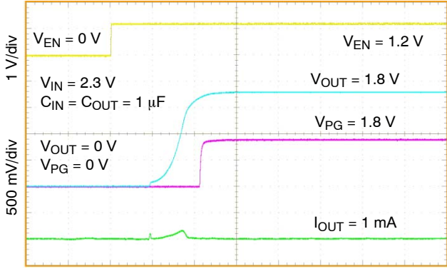
Figure 23. Turn-On Response After Asserting EN NCV8752A, V_{OUT} = 1.8 V
