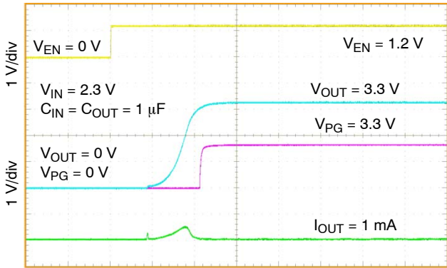
Figure 25. Turn-On Response After Asserting EN NCV8752A, V_{OUT} = 3.3 V
