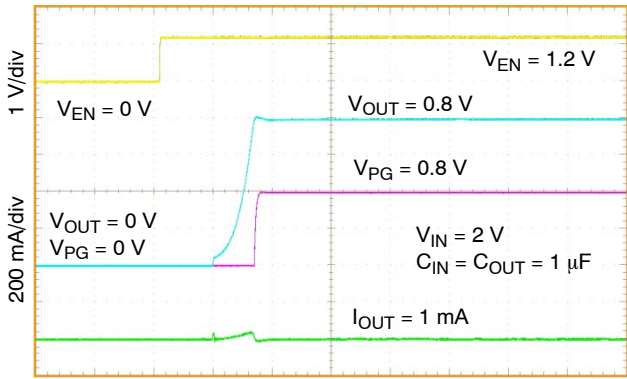
Figure 21. Turn-On Response After Asserting EN NCV8752A, V_{OUT} = 0.8 V
