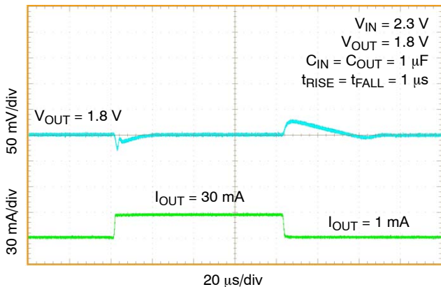
Figure 9. Load Transient Response, 1 mA – 30 mA NCV8752A/B, V_{OUT} = 1.8 V
