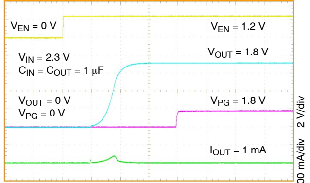
Figure 24. Turn-On Response After Asserting EN NCV8752B, V_{OUT} = 1.8 V
