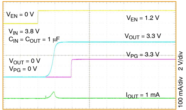
Figure 26. Turn-On Response After Asserting EN NCV8752B, V_{OUT} = 3.3\text{ V}
