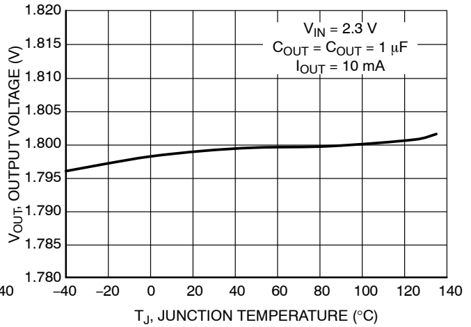
Figure 58. Output Voltage vs. Temperature V OUT = 1.8 V
