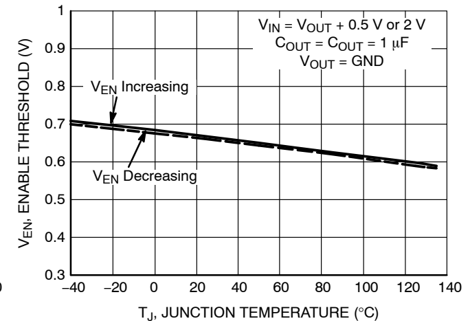
Figure 68. Enable Threshold vs. Temperature
