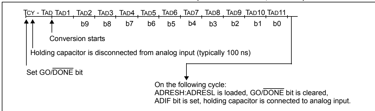
FIGURE 20-3: A/D CONVERSION TAD CYCLES ( \text{ACQT}\langle 2:0 \rangle = 000, \text{TACQ} = 0 )
