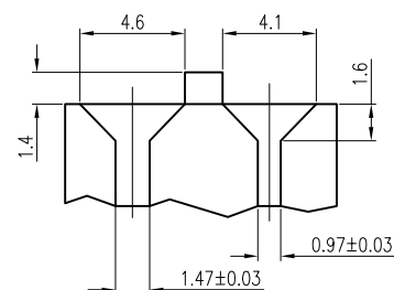
DETAIL-3: MATING SLOTS
