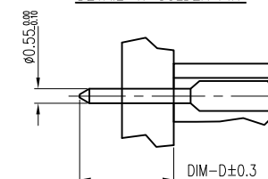
DETAIL-1: SOLDER PIN
