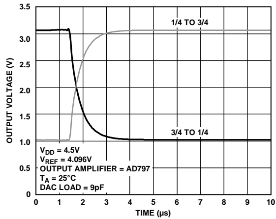
Figure 25. Settling Time
