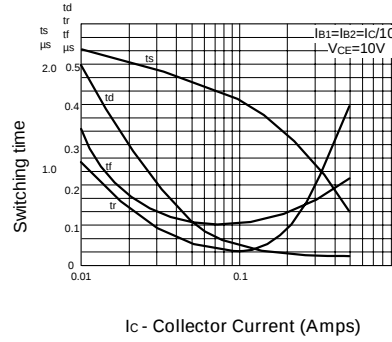
Switching Speeds
