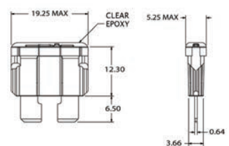
Dimensions SMART GLOW ATO®
