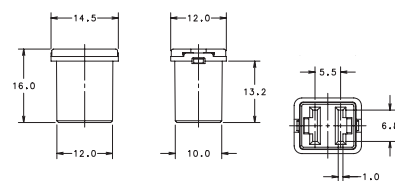
Dimensions Low Profile JCASE®
