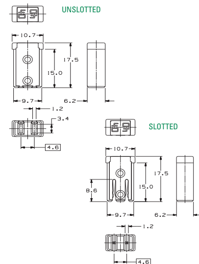
Dimensions MCASE+®
