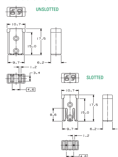
Dimensions MCASE+®
