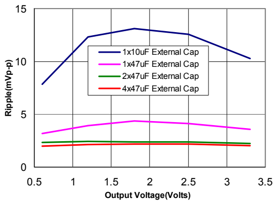
Figure 36. Output ripple voltage for various output voltages with external 1x10 μF, 1x47 μF, 2x47 μF or 4x47 μF ceramic capacitors at the output (12A load). Input voltage is 5V.
