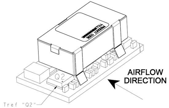
Figure 46. Preferred airflow direction and location of hot-spot of the module ( T_{ref} ).
