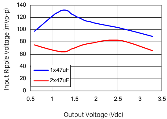
Figure 34. Input ripple voltage for various output voltages with 1 \times 47\mu F or 2 \times 47\mu F ceramic capacitors at the input (12A load). Input voltage is 5V.
