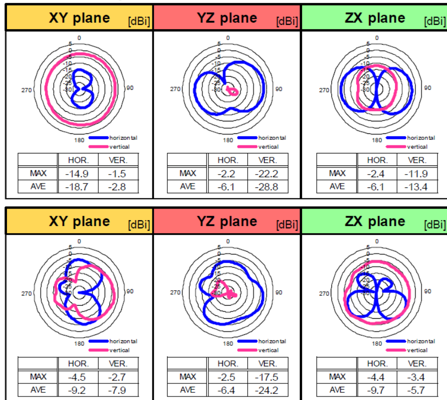
Figure 15 – Directivity for 1MW M.2 Module Standalone
