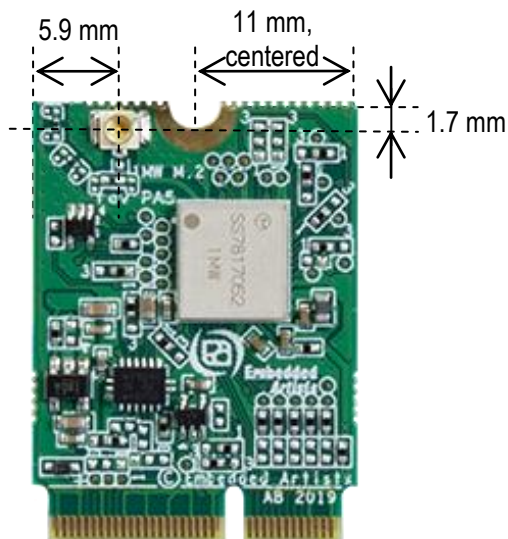
Figure 2 – M.2 Module With, and Without, Trace Antenna
