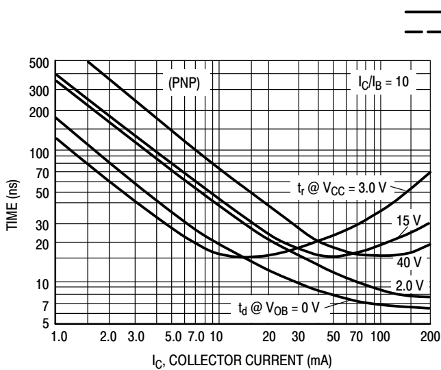
Figure 22. Turn-On Time
