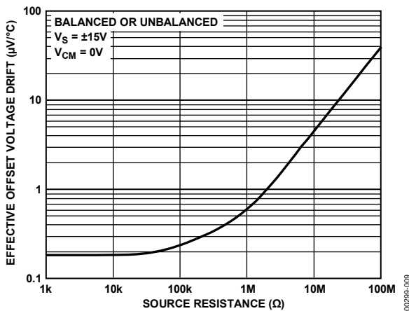
Figure 9. Effective TCV_{0S} vs. Source Resistance
