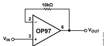
Figure 33. Unity-Gain Follower
