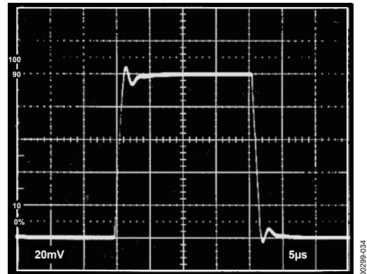
Figure 34. Small Signal Transient Response with Overcompensation ( C_{LOAD} = 1000 \text{ pF} , A_{VCL} = 1 , C_{OC} = 220 \text{ pF} )
