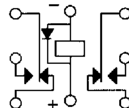
TERMINAL VIEW
