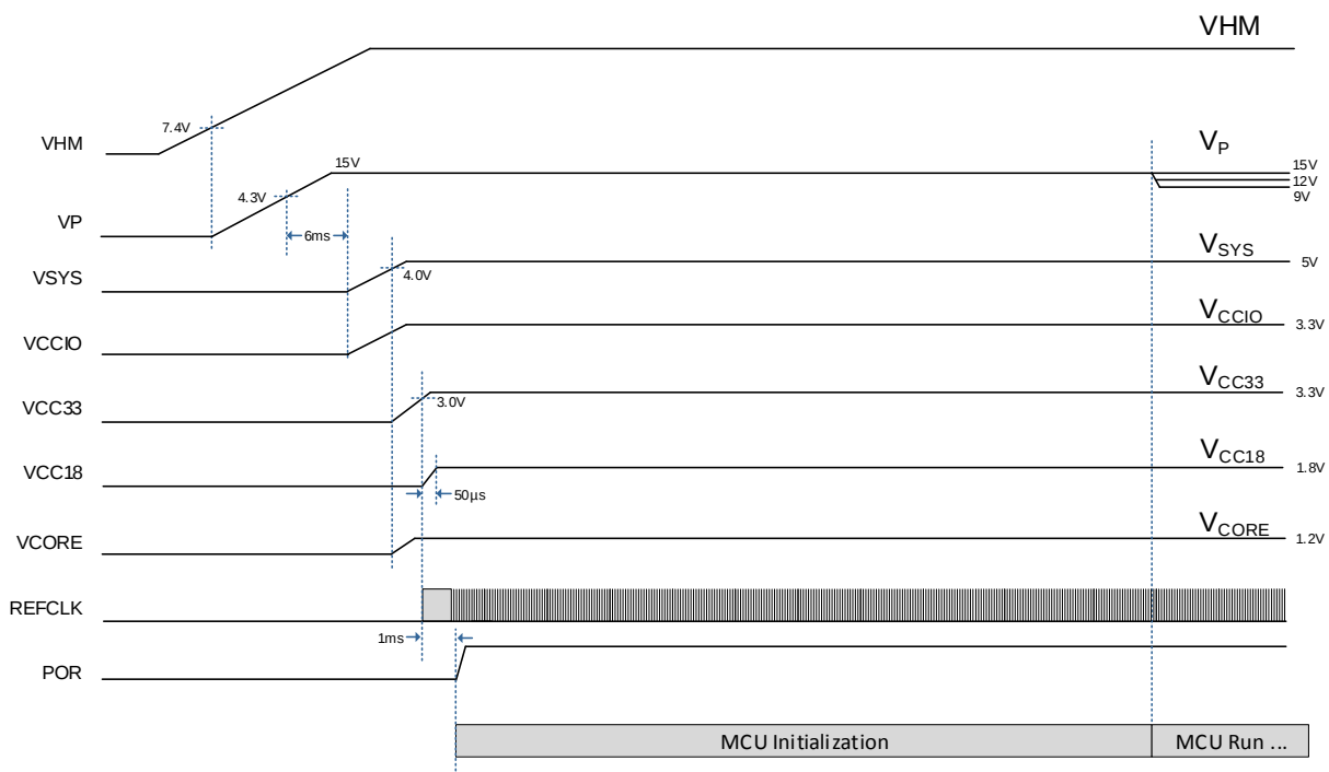
Figure 10-6 Power-Up Sequence
