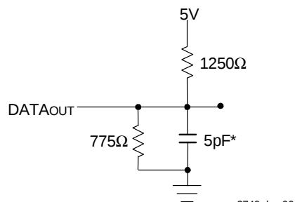
Figure 2. Output Test Load (for t_{LZ} , t_{HZ} , t_{WZ} , t_{OW} )
