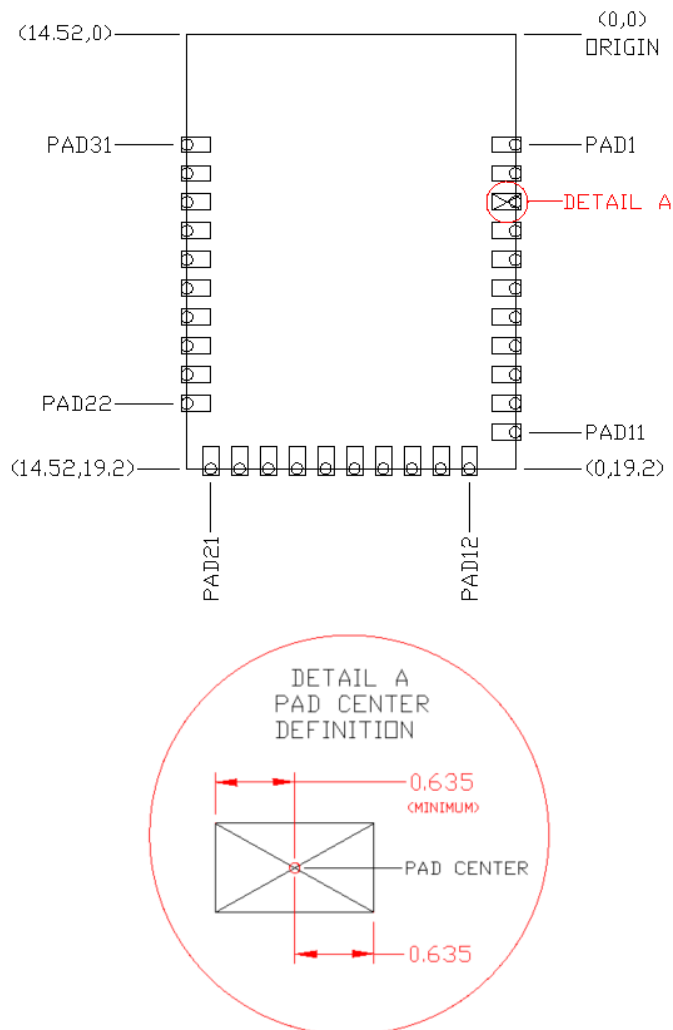
Figure 6. Solder Pad Reference Location
