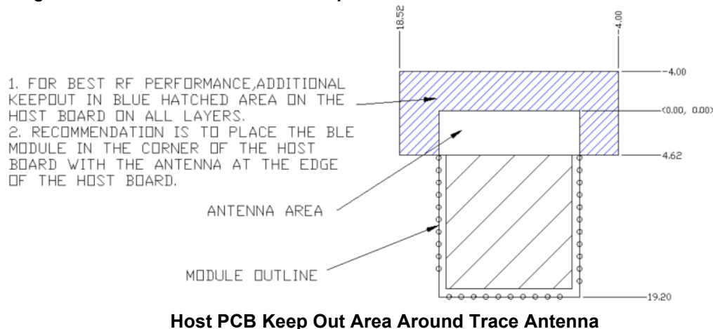
Figure 3. Recommended Host PCB Keep Out Area Around the CYBLE-012011-00 Antenna
