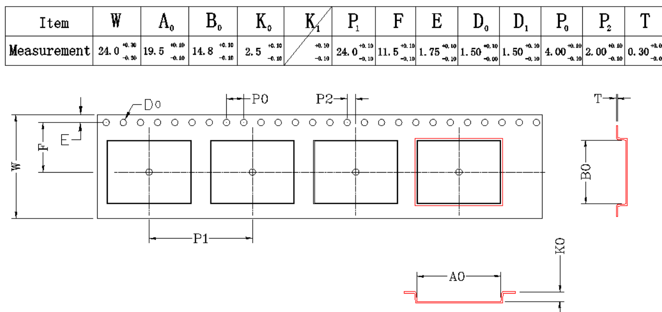
Figure 10. CYBLE-012011-00 Tape Dimensions
