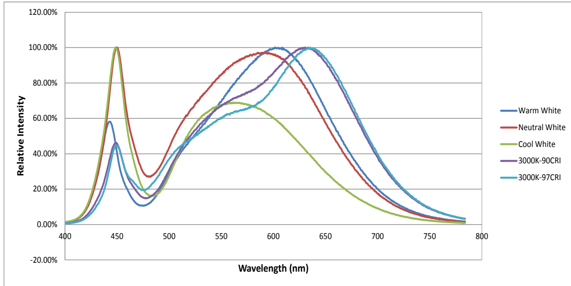
Typical Spectrum
