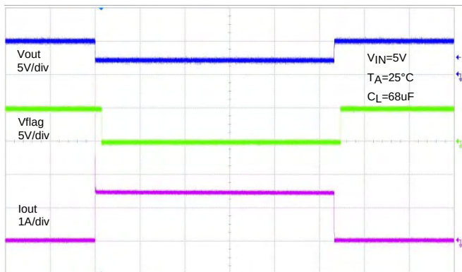
20ms/div Channel 1 Short Circuit with Blanking Time and Recovery
