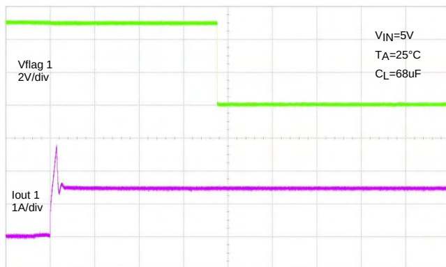
2ms/div Channel 1 1 \Omega Load Connected to Enabled Device
