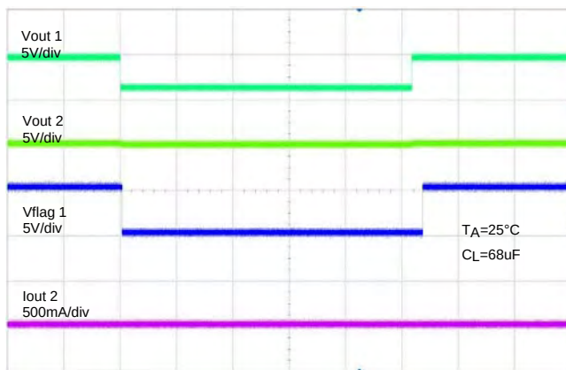
100ms/div Channel 1 Enabled and Shorted with Channel 2 Disabled
