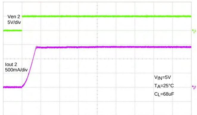
500 \mu s/div Channel 2 Short Circuit Current, Device Enabled Into Short
