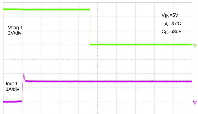
2ms/div Channel 1 2 \Omega Load Connected to Enabled Device
