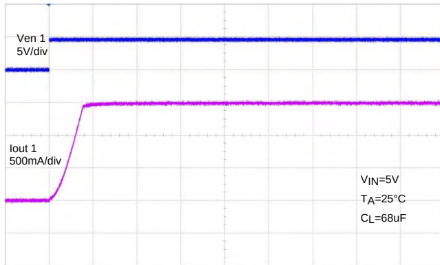
500 \mu s/div Channel 1 Short Circuit Current, Device Enabled Into Short
