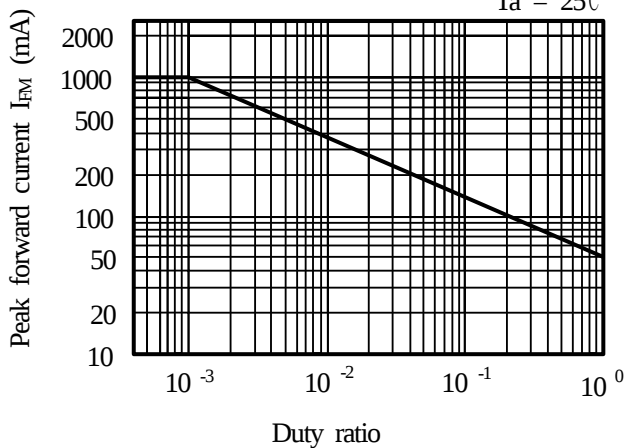
(Fig.7) Forward current vs. duty ratio
