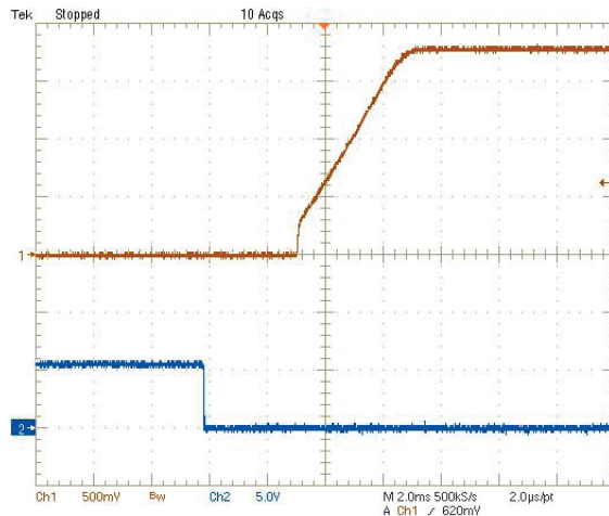
On/Off Enable Delay (Vin=12V, Vout=1.8V, Iout=20A, Cload=188μF) Trace2=Enable, 5V/div Trace1=Vout, 500mV/div
