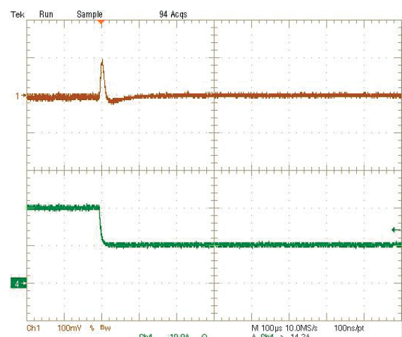
Step Load Transient Response (Vin=12V, Vout=3.3V, Cload=188μF, Iout=20A to 10A) Trace 1=Vout, 100 mV/div(AC), Trace 4=Iout, 10A/div.
