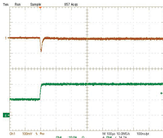
Step Load Transient Response (Vin=12V, Vout=1.8V, Cload=188μF, Iout=10A to 20A) Trace 1=Vout, 100 mV/div(AC), Trace 4=Iout, 10A/div.
