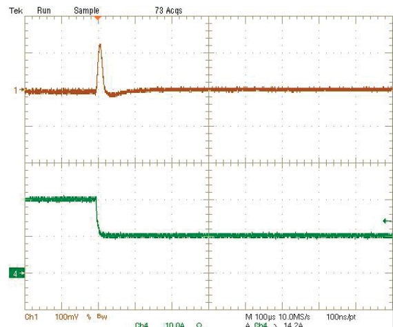
Step Load Transient Response (Vin=12V, Vout=1.8V, Cload=188μF, Iout=20A to 10A) Trace 1=Vout, 100 mV/div(AC), Trace 4=Iout, 10A/div.
