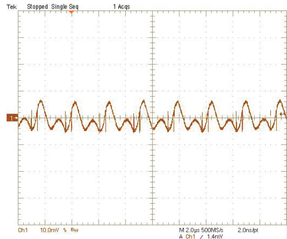
Output Ripple and Noise (Vin=12V, Vout=1.8V, Iout=20A, Cload=188μF, ScopeBW=20MHz) Trace1=Vout, 10mV/div(AC)
