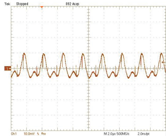
Output Ripple and Noise (Vin=12V, Vout=3.3V, Iout=20A, Cload=188μF, ScopeBW=20MHz) Trace1=Vout, 10mV/div(AC)
