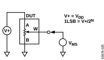
Figure 27. Potentiometer Divider Nonlinearity Error (INL, DNL)
