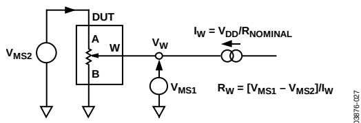
Figure 29. Wiper Resistance
