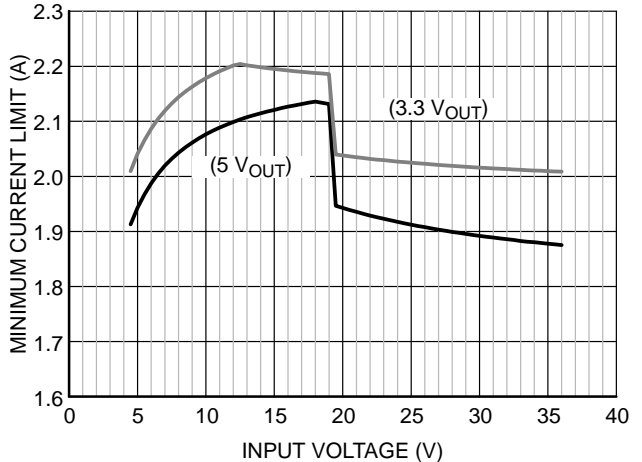
Figure 26. NCV890204 Load Current Capability with 4.7 \mu H Inductor
