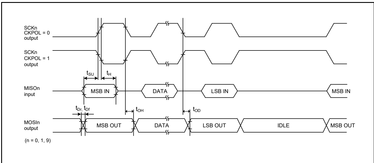
Figure 2.44 SCKn CKPOL = 0 and CKPOL = 1 outputs, MISO input, and MOS output timing (master, CKPH = 1)
