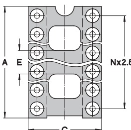
INSULATOR
